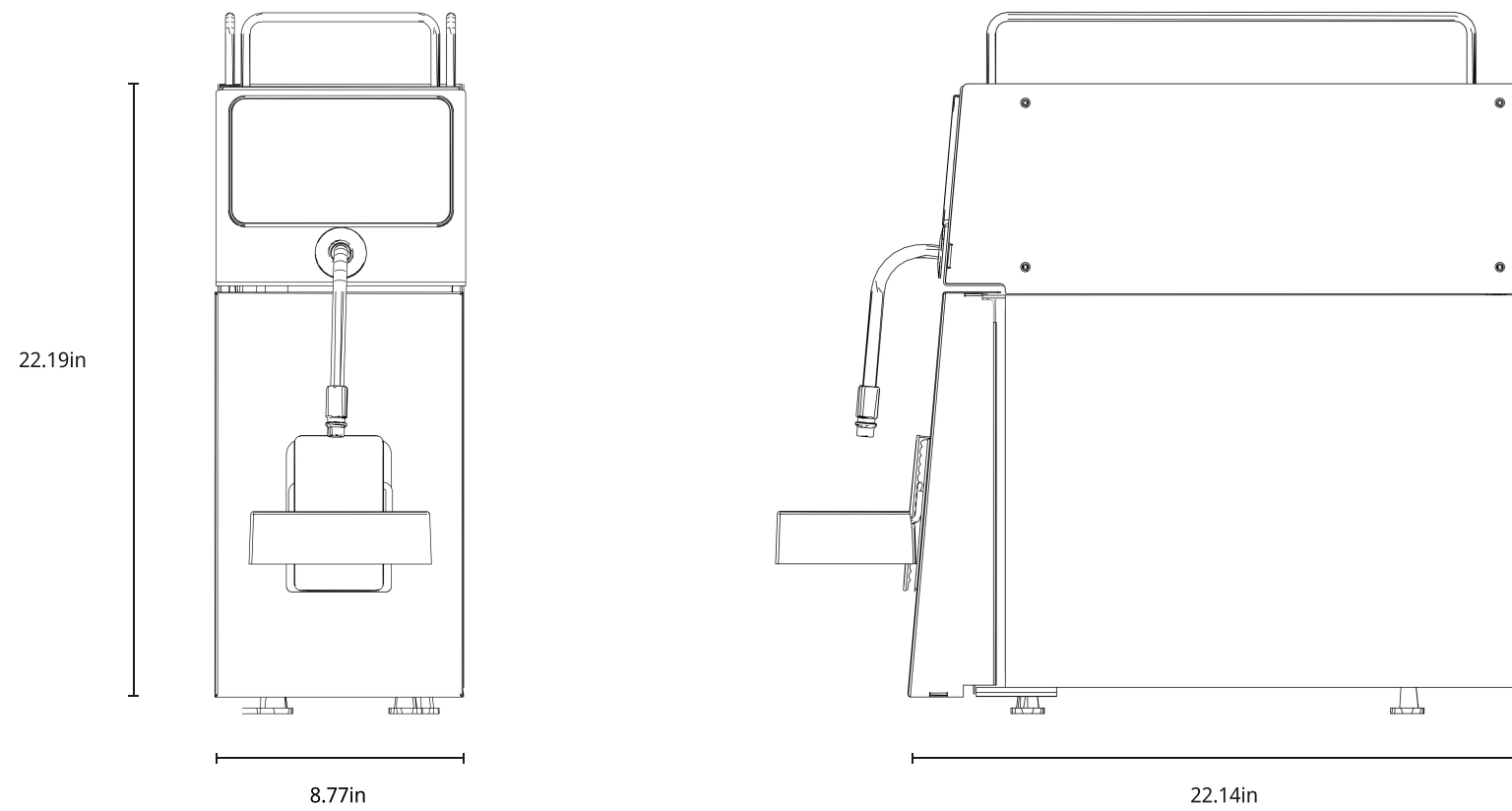
Dimensions (WxHxD): 8.77 x 22.19 x 22.14 inches and with Accessories 8.77 x 24.70 x 26.80 inches
